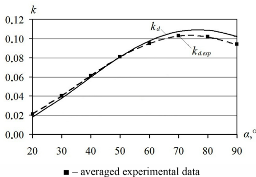
Fig. 1. Dependence: destruction coefficient k_d – angle of attack \alpha
