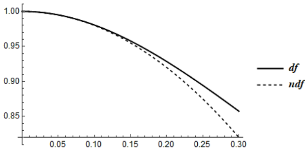
Fig. 3. Graphs of the differential of a function and its expansion in a Maclaurin series
