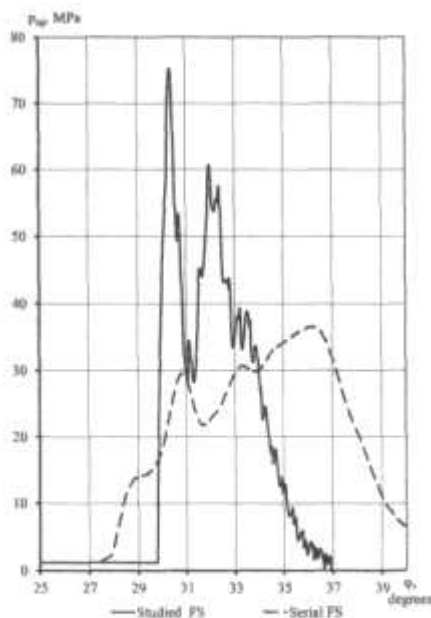
Fig. 2. Dependence of fuel injection pressure on angle of rotation of the cam shaft of the high-pressure pump at n_{L,sk} = 1,600 \text{ min}^{-1}
