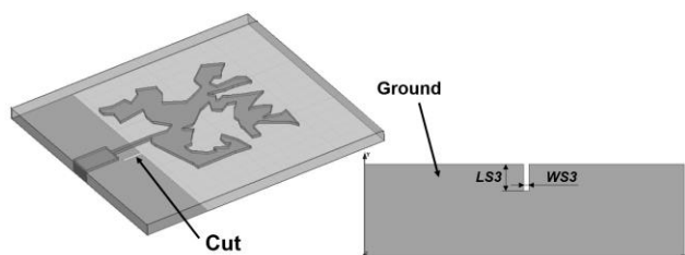
Fig. 10. The ground screen with a cutout.
