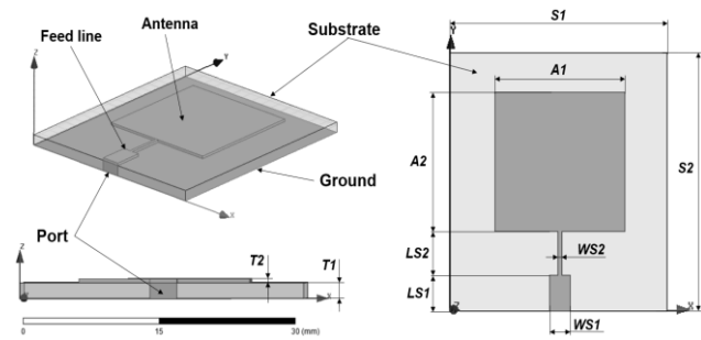
Fig. 2. Square printed antenna adopted as a reference for comparison.
