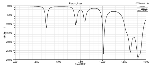
Fig. 3. Frequency dependence of RL of a square printed antenna.
