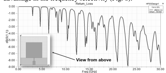
Fig. 8. Frequency dependence of RL of the square antenna, located end-to-end with ground. ( G2 = 9.07697 mm).
