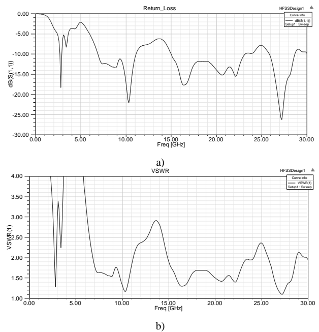
Fig. 7. Frequency dependences for an antenna with ground, which ends with the projection of the antenna ( G2 = 9.077 mm): a) – RL, b) – VSWR.
