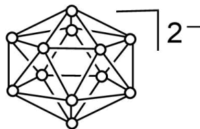
Fig. 1. [\text{B}_{12}\text{H}_{12}]^{2-} structure
