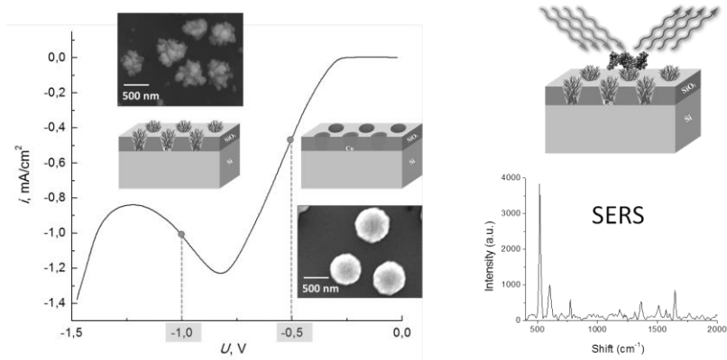
Fig. 1. Control of the shape of Cu nanostructures in pores of \text{SiO}_2 matrixes on single-crystal silicon substrate at electrodeposition process and surface enhanced Raman spectrum of the Rhodamine 6G aqueous solution with a concentration of 10^{-6} M on the copper dendritic nanostructures
