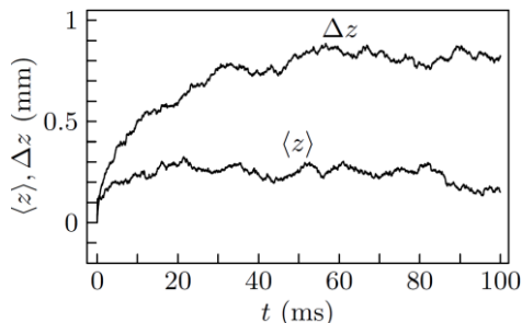
Fig. 1. Average coordinate and r.m.s. deviation of 100 Na atoms vs. time
