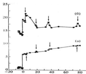
Fig. 1. Dependence of polymorphic forms of ice on pressure [1].
