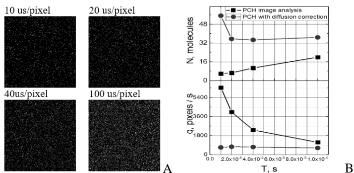
Fig. 1. Fluorescence images (a stack of 100 128x128 images) of purified GFP in buffer with various dwell time (10, 20, 40, and 100 μs/pixel) (A) and results of PCH analysis with diffusion correction (B)
